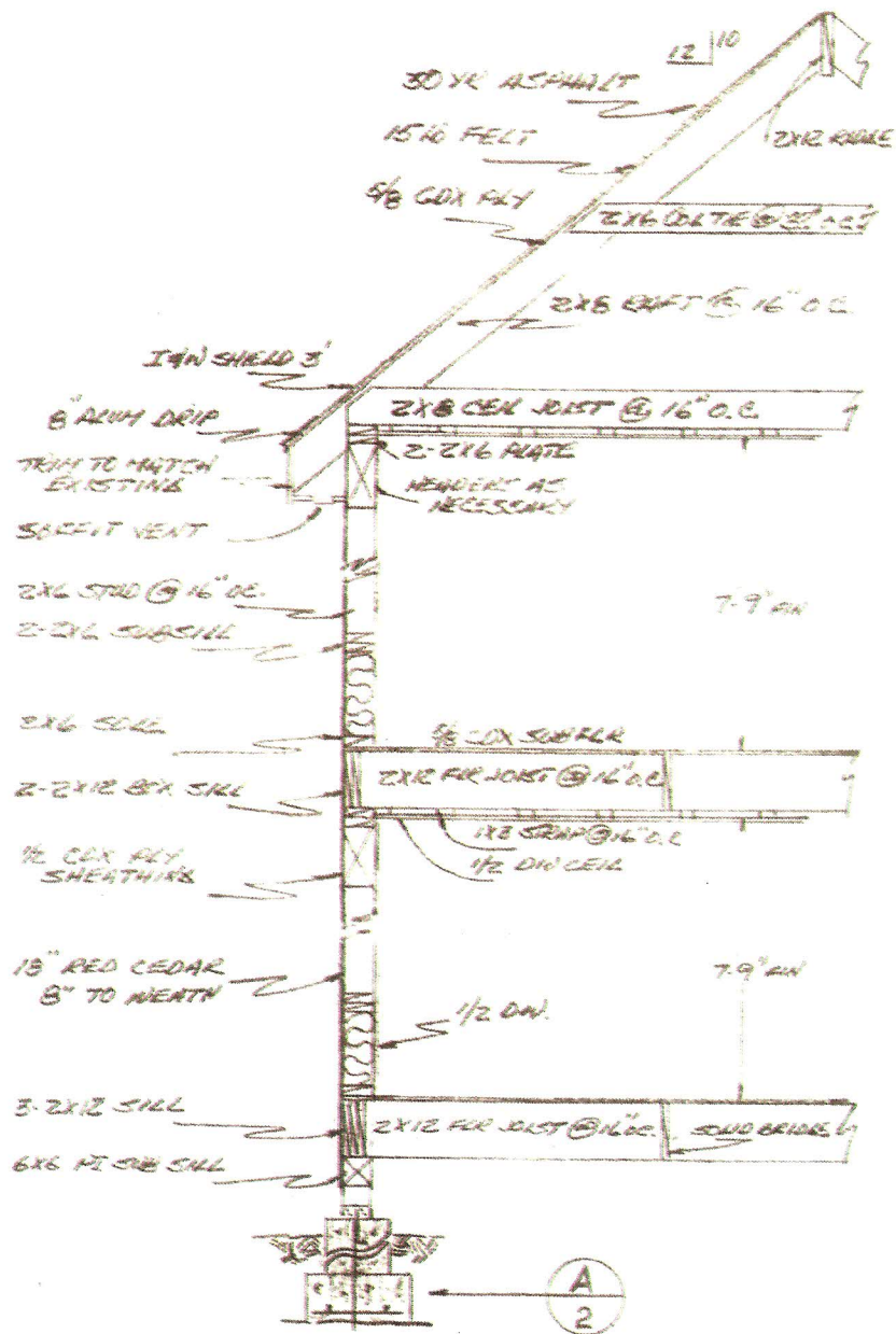
TYPICAL WALL SECTION SCALE 3/8" = 1'-0"
